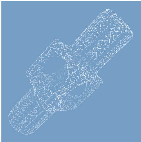
(c) EMST of tangent plane centers o_i
