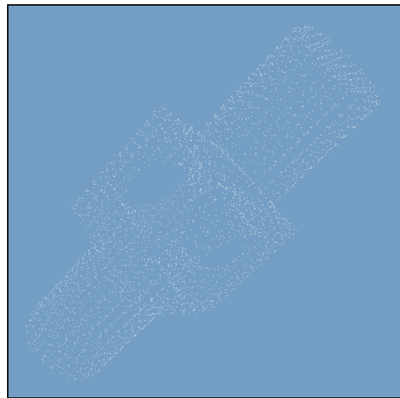
(b) Sampled points (x_i) ( n = 4102 )
